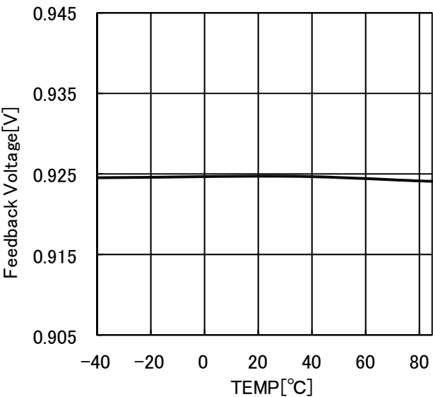
Fig.7 Feedback voltage
