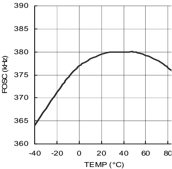
Fig.9 Operating Frequency
