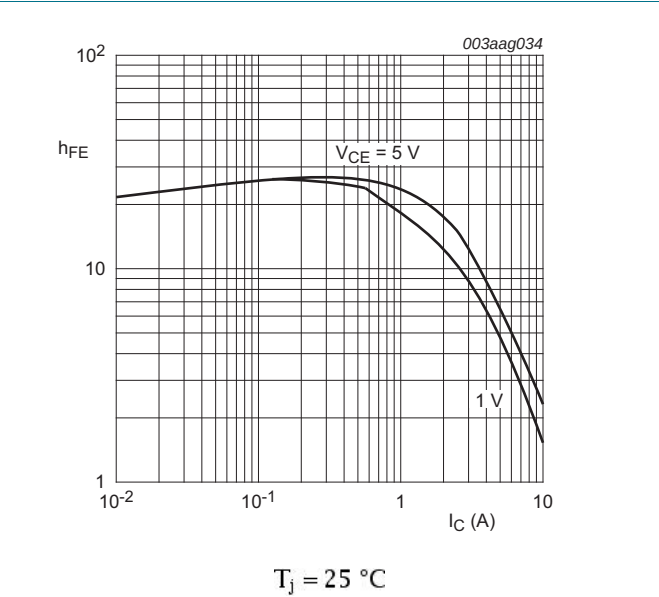
Fig 11. DC current gain as a function of collector current; typical values
