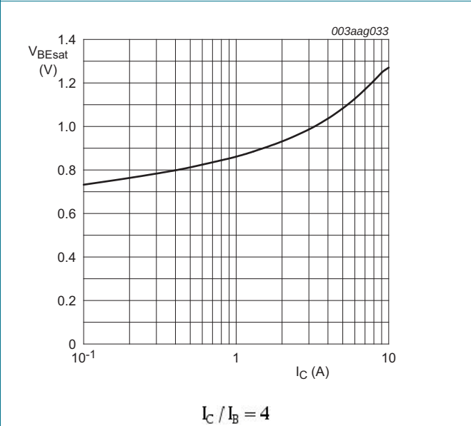
Fig 10. Base-emitter saturation voltage as a function of collector current; typical values
