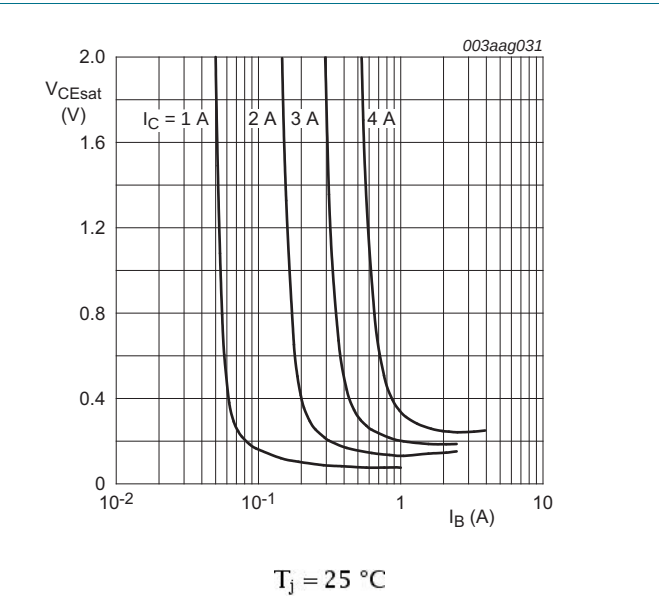
Fig 9. Collector-emitter saturation voltage as a function of base current; typical values
