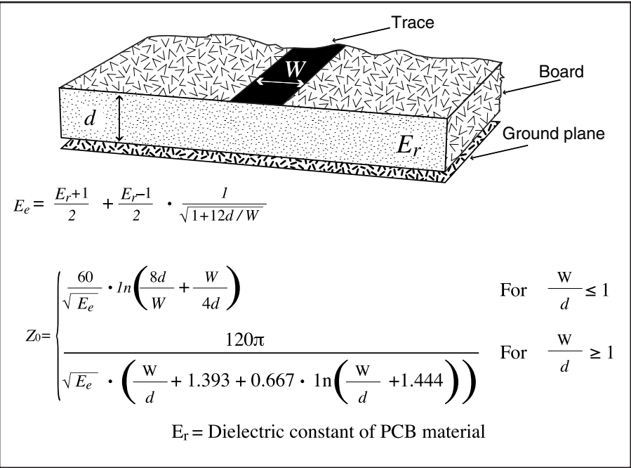
Figure 8: Microstrip Formulas
