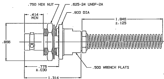
FIG 2 -9 SHOWN
