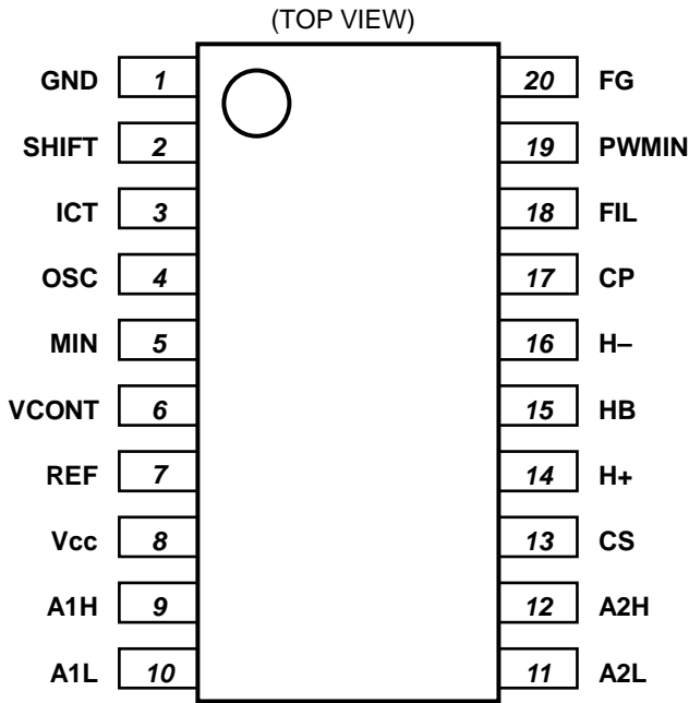
Fig.1 Pin configuration
