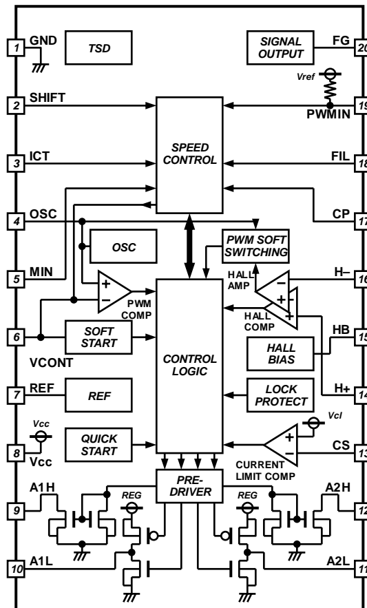
Fig.2 Block diagram
