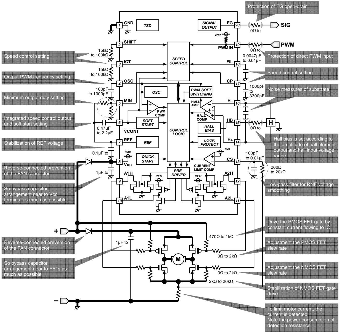
Fig.33 PWM controllable 4 wires type motor application circuit
