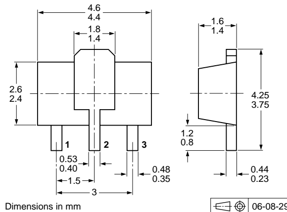
Fig 18. Package outline SOT89 (SC-62/TO-243)
