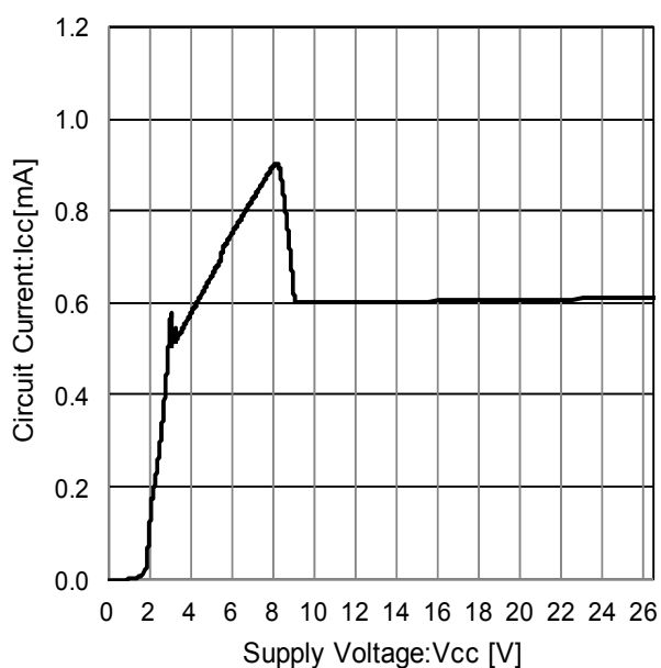
Figure 59. Circuit Current
