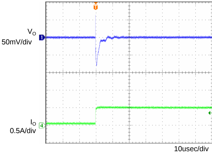
Fig.4 Transient Response (0→0.5A) Co=1µF, T_a = 25^\circ\text{C}
