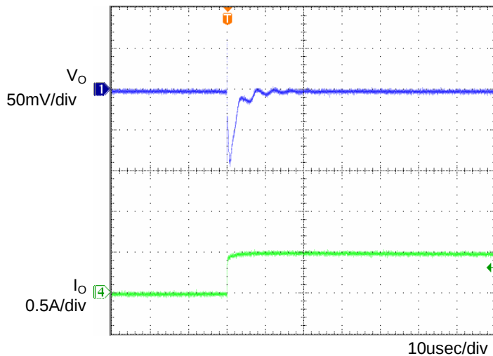
Fig.5 Transient Response (0→0.5A) Co=1µF, T_a = 105^\circ\text{C}
