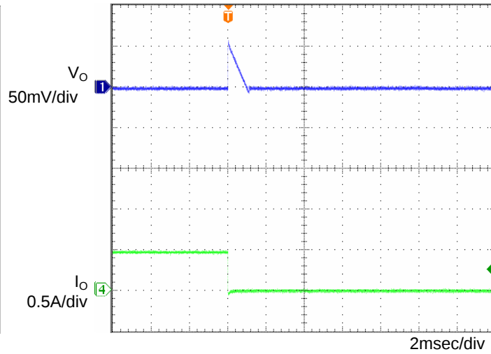
Fig.6 Transient Response (0.5→0A) Co=1µF, T_a = -40^\circ\text{C}
