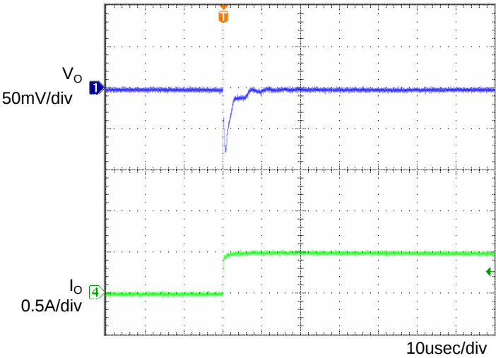
Fig.3 Transient Response (0→0.5A) Co=1µF, T_a = -40^\circ\text{C}
