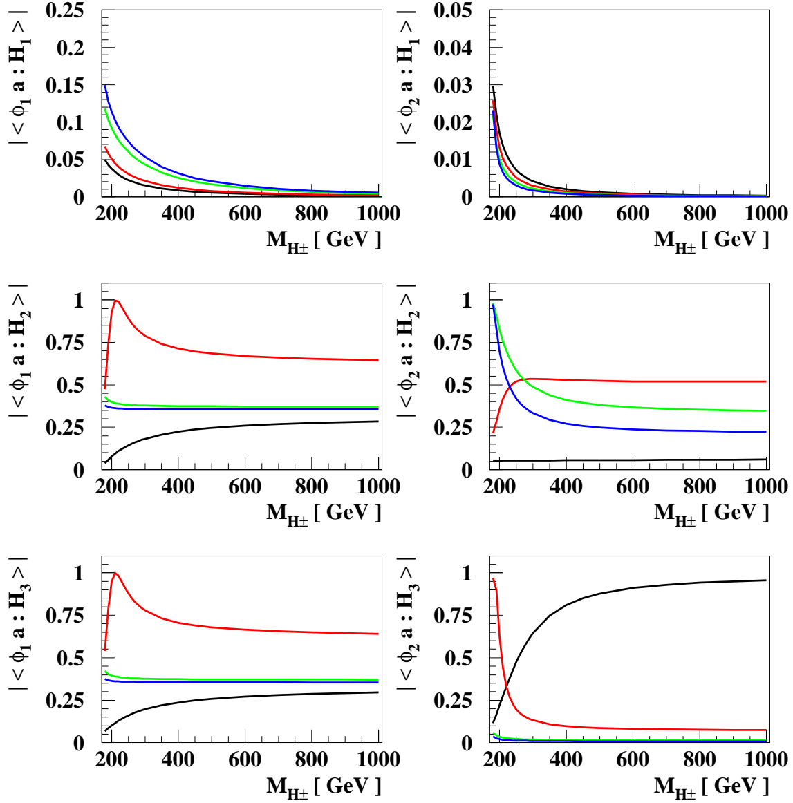
Figure 16: The magnitudes of the mixing quantities |\langle \phi_{1a} : H_i \rangle| (left) and |\langle \phi_{2a} : H_i \rangle| (right), defined in (37), as functions of M_{H^\pm} for M_S = 10 TeV and \Phi_A = 10^\circ . The black, red, green and blue lines are for \tan \beta = 5, 10, 30 and 50 , respectively.
