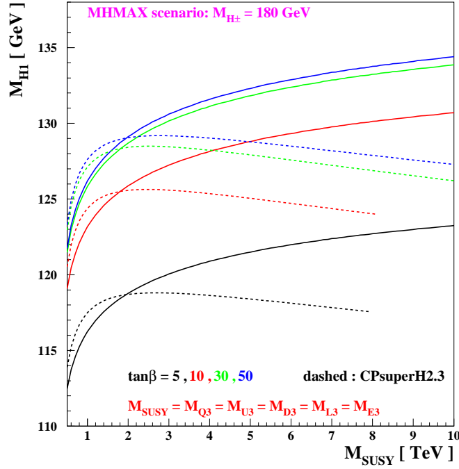
Figure 3: The lightest Higgs mass calculated in the MHMAX scenario using CPsuperH3.0 (solid lines) and CPsuperH2.3 (dashed lines) as functions of M_S = M_{Q3} = M_{U3} = M_{D3} = M_{L3} = M_{E3} for M_{H^\pm} = 180 GeV, \mu = 200 GeV and various values of \tan\beta .
