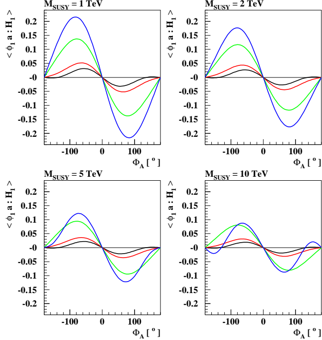
Figure 10: The CP mixing quantity \frac{2O_{\phi_1 1} O_{a1}}{O_{\phi_1 1}^2 + O_{a1}^2} for the lightest mass eigenstate H_1 in scenarios with M_{H^\pm} = 500 GeV and M_S = 1 TeV (upper left), M_S = 2 TeV (upper right), M_S = 5 TeV (lower left), M_S = 10 TeV (lower right). The black, red, green and blue lines are for \tan \beta = 5, 10, 30 and 50 , respectively.
