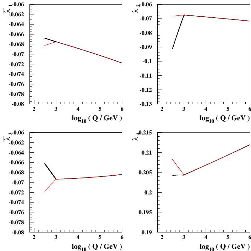
Figure 1: The black lines show the one-loop running of the 2HDM quartic couplings for Q < 10^6 GeV, assuming M_{H^\pm} = 300 GeV and \tan\beta = 5 . The other input parameters are given in Eq. (34). The thin red lines show the running of -(g^2 + g'^2)/8 , -(g^2 - g'^2)/4 , and g^2/2 in the panels for \bar{\lambda}_{1,2} , \bar{\lambda}_3 , and \bar{\lambda}_4 , respectively.
