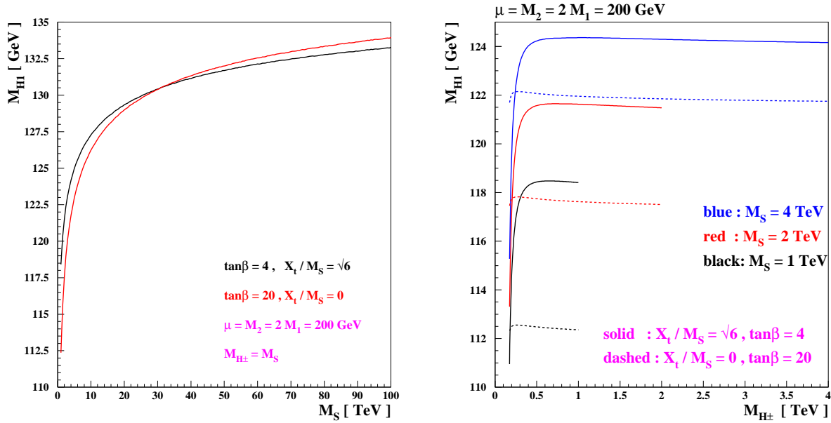
Figure 7: Left panel: Calculations of M_{H_1} made using CPsuperH3.0 for M_{H^\pm} = M_S \leq 100 TeV, assuming \tan\beta = 4 and X_t/M_S = \sqrt{6} (black line) and \tan\beta = 20 and X_t/M_S = 0 (red line) both for the case \mu = M_2 = 2M_1 = 200 GeV. Right panel: calculations of M_{H_1} as a function of m_{H^\pm} made using CPsuperH3.0 over the range M_{H^\pm} \in [m_t, M_S] for M_S = 1, 2 and 4 TeV (black, red and blue lines, respectively), also for the two cases X_t/M_S = \sqrt{6} and \tan\beta = 4 (solid lines) and X_t/M_S = 0 and \tan\beta = 20 (dashed lines) and \mu = M_2 = 2M_1 = 200 GeV. These results can be compared with those of [35].
