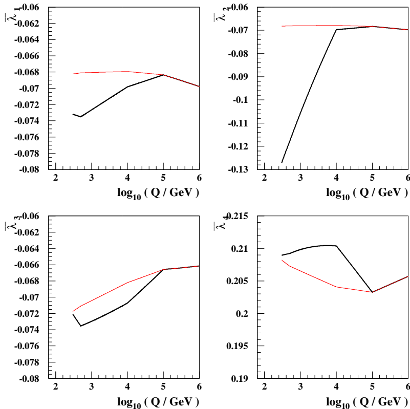
Figure 2: The same as in Fig. 1, but for an hierarchical scenario with \rho = 10 and input parameters given in Eq. (35).
