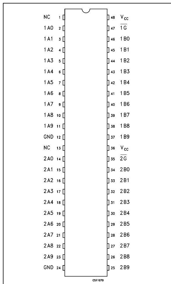
Figure 1: Pin Connection
