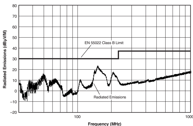
Radiated Emissions EN 55022 Class B, 10 Meters Converter Output = \pm 15\text{Vdc} @ \pm 132\text{mA}
