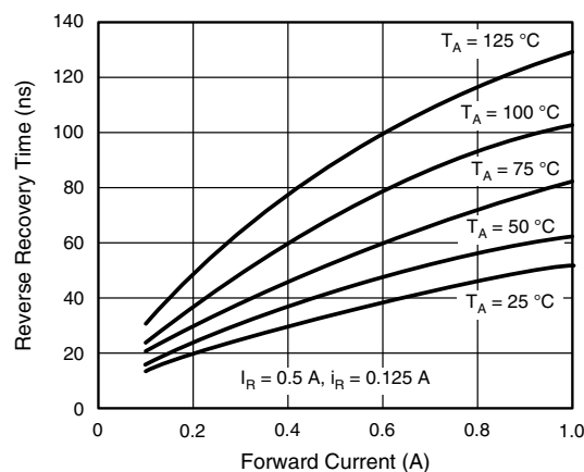
Fig. 6 - Max. Reverse Recovery Time vs. Forward Current
