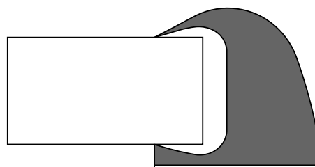
Too much solder Pad geometry too large
