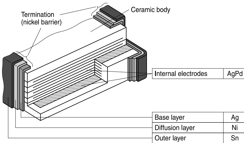
Multilayer CTVS: Structure of nickel barrier termination
