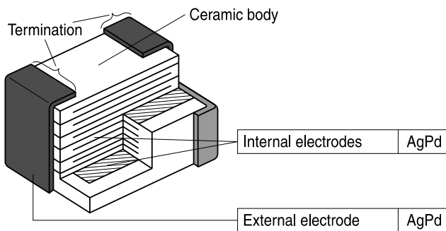
Multilayer varistor: Structure of silver-palladium termination
