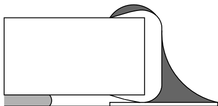
Good solder joint
