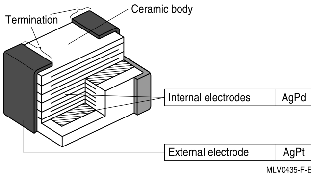
Multilayer varistor: Structure of silver-platinum termination
