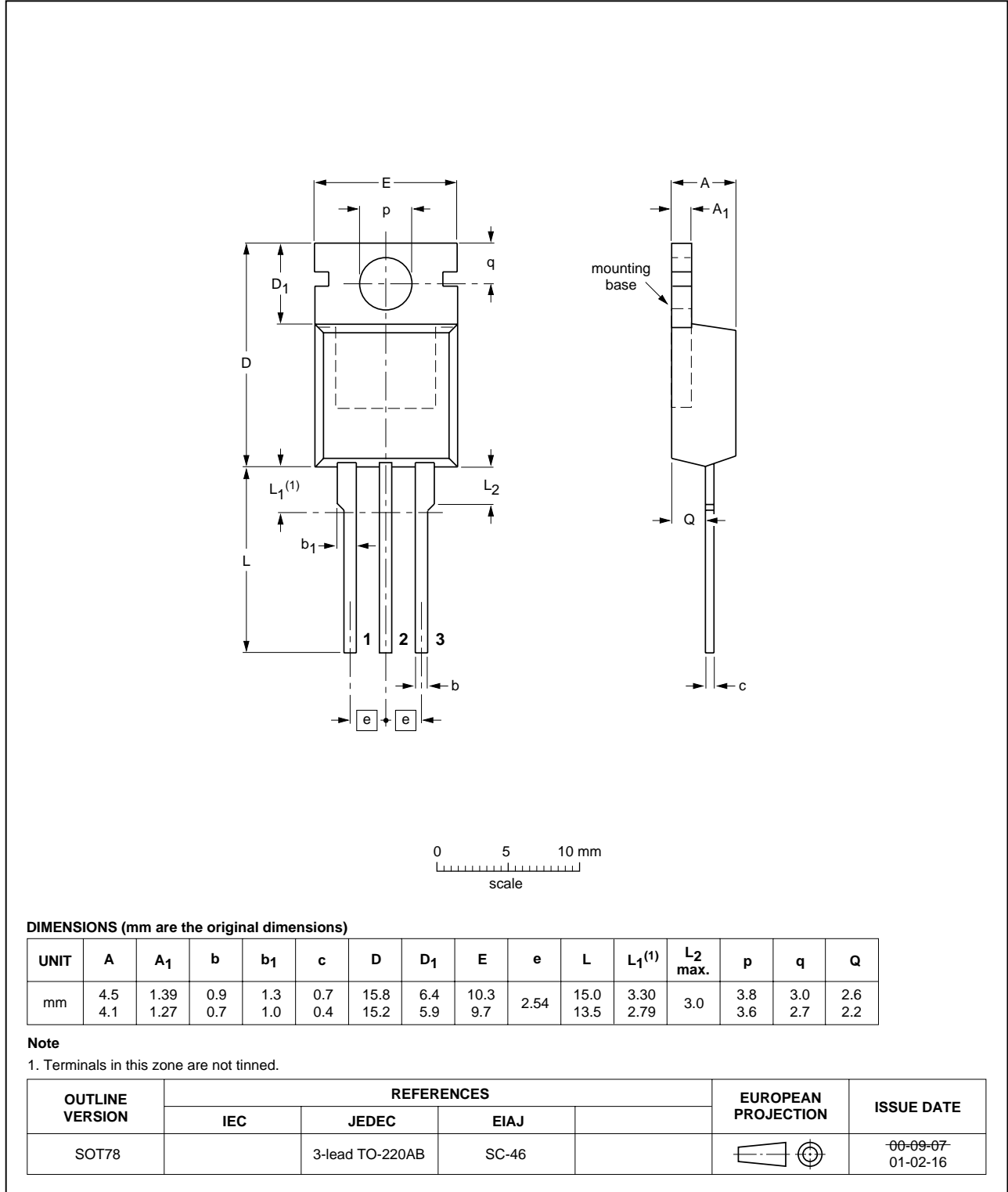
Fig 16. SOT78 (TO-220AB).
