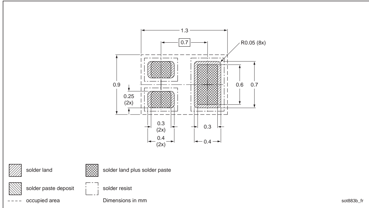
Fig 8. Reflow soldering footprint DFN1006B-3 (SOT883B)
