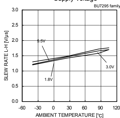
Fig.90 Slew Rate L-H – Ambient Temperature
