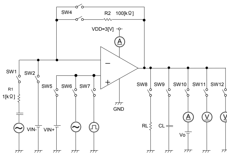
Fig.186 Test circuit 2
