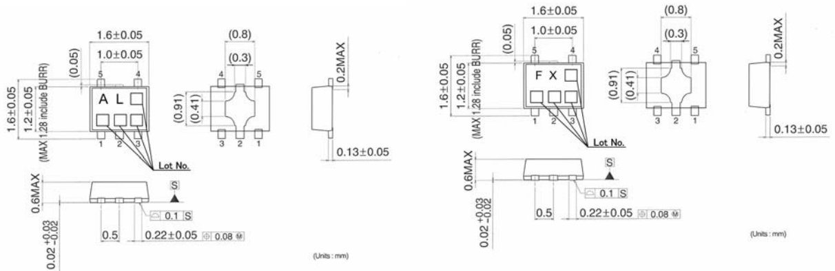
BU7445HFV (HVS0F5) (Unit : [mm])
