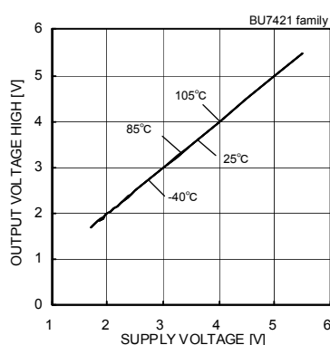
Fig.120 Output Voltage High - Supply Voltage ( R_L=10[k\Omega] )
