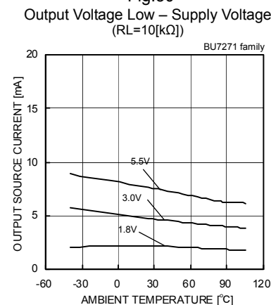
Output Source Current – Ambient Temperature (VOUT=VDD-0.4[V])
