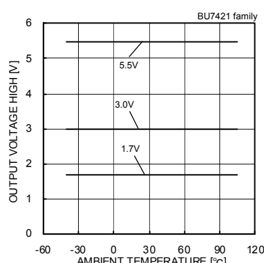
Fig.121 Output Voltage High - Ambient Temperature ( R_L=10[k\Omega] )
