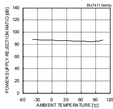
Fig.112 Power Supply Rejection Ratio – Ambient Temperature
