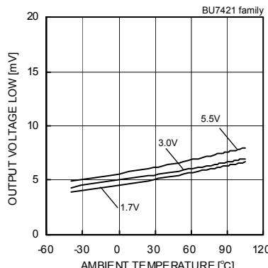
Fig.123 Output Voltage Low - Ambient Temperature ( R_L=10[k\Omega] )
