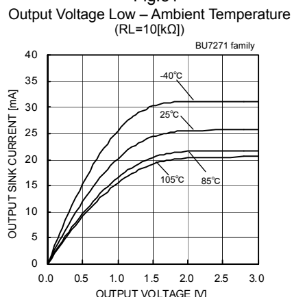
Output Sink Current – Output Voltage (VDD=3[V])
