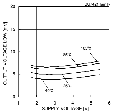
Fig.122 Output Voltage Low - Supply Voltage ( R_L=10[k\Omega] )
