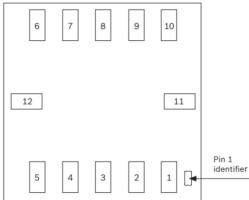
Pin configuration for SPI interface (bottom view)
