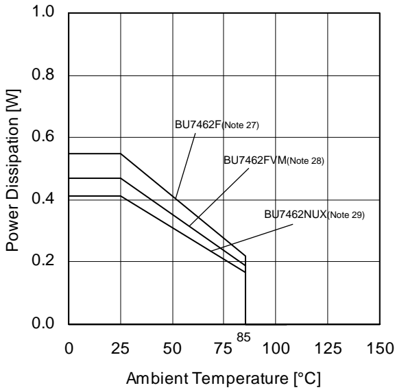
(e) BU7462xxx
