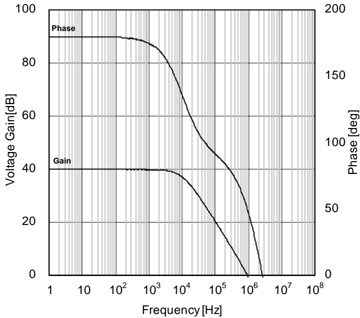
Figure 70. Voltage Gain · Phase vs Frequency
