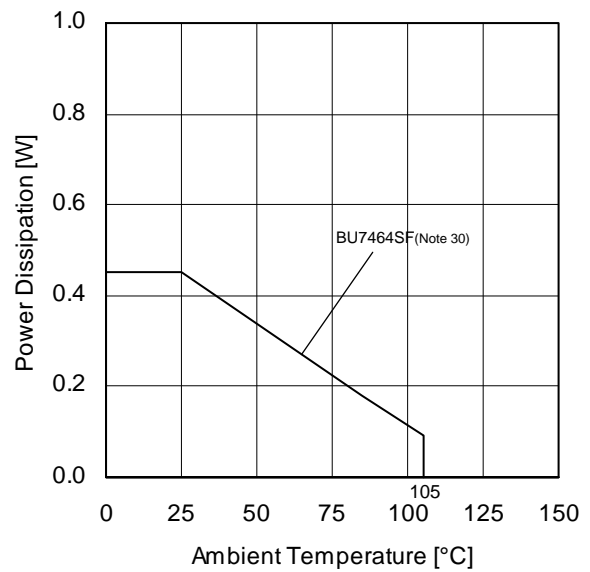
(h) BU7464SF
