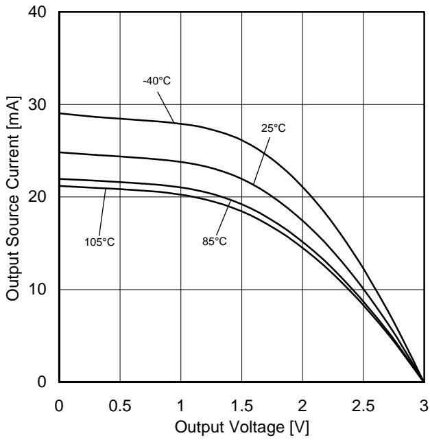
Figure 33. Output Source Current vs Output Voltage (VDD=3V)
