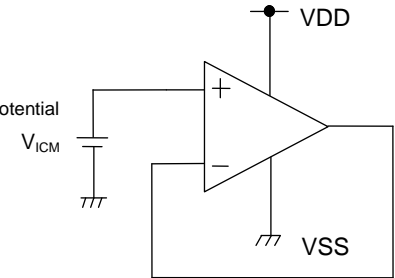
Figure 79. Example of Application Circuit for Unused Op-amp
