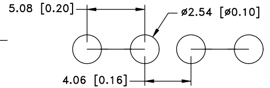
MOUNTING DETAIL FOR 2 CLIPS
