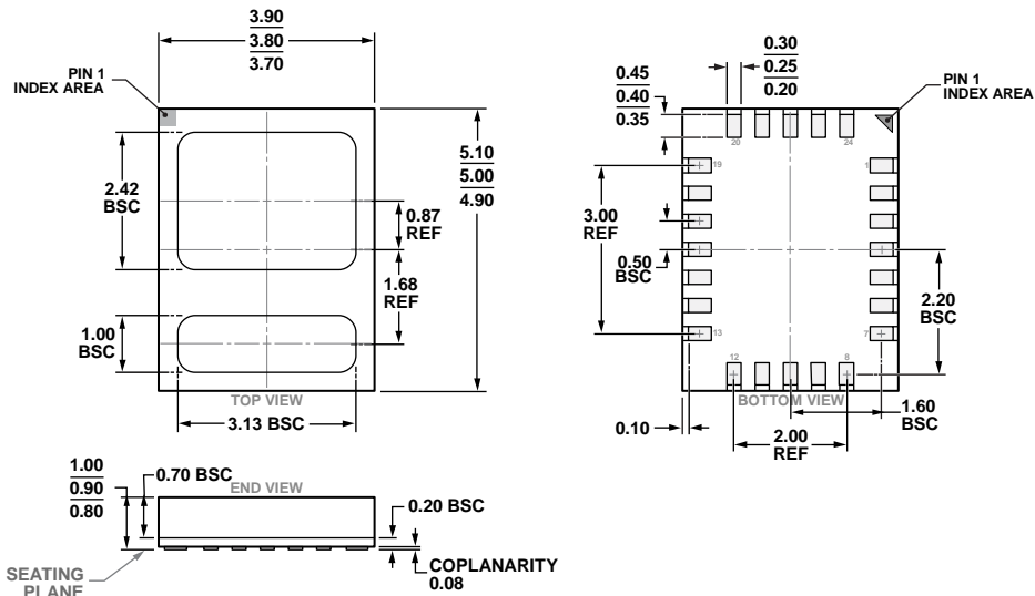
Figure 41. 24-Terminal Chip Array Small Outline No Lead Cavity [LGA_CAV] 3.80 mm x 5.00 mm Body and 0.9 mm Package Height (CE-24-1) Dimensions shown in millimeters
