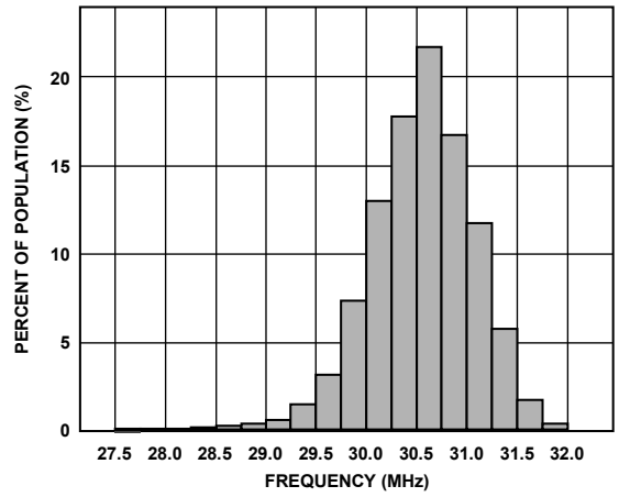
Figure 8. 32 MHz Clock Frequency Distribution; Default Settings; Before User Calibration, Register 0x4D = 0x425E
