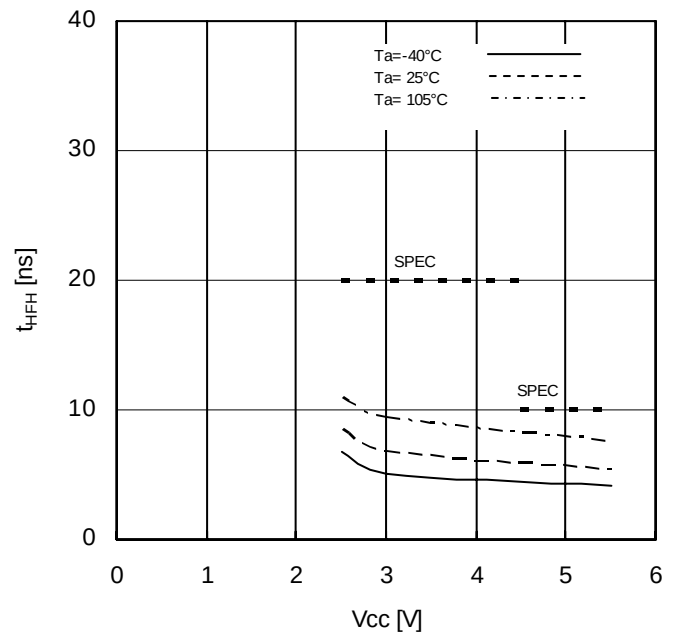
Figure 24. HOLDB Setting Hold Time vs Supply Voltage
