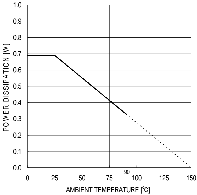
Figure 1 Derating curve
