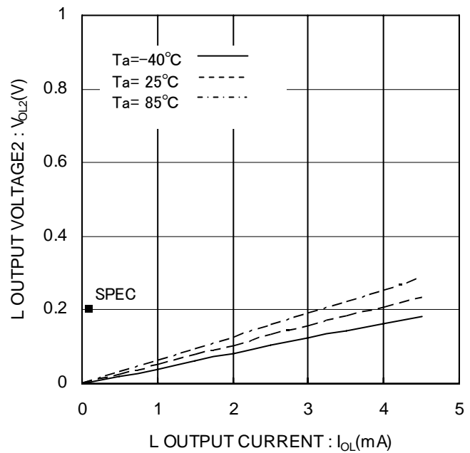
Figure 7. "L" output voltage2 V O2 (VCC=1.7V)
