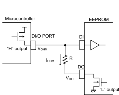
Figure 53. Circuit at DI, DO direct connection (Microcontroller DI/O "H" output, EEPROM "L" output)
