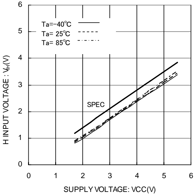
Figure 4. "H" input voltage V IH (CS,SK,DI,ORG)
