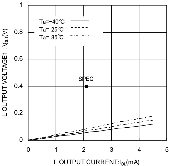
Figure 6. "L" output voltage1 V O1 (VCC=2.7V)
