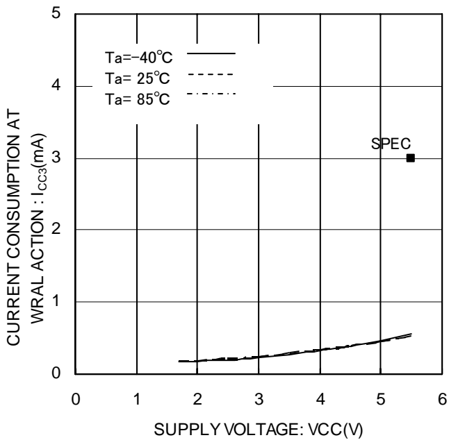
Figure 18. Current consumption at WRAL action I_{CC3}(WRAL, f_{SK}=3MHz)
