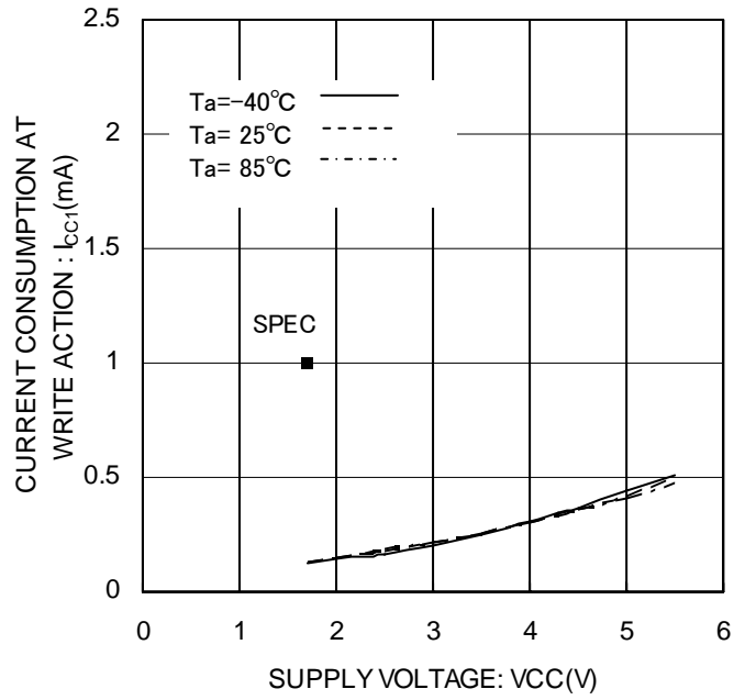
Figure 13. Current consumption at WRITE action I_{CC1}(WRITE, f_{SK}=1MHz)
