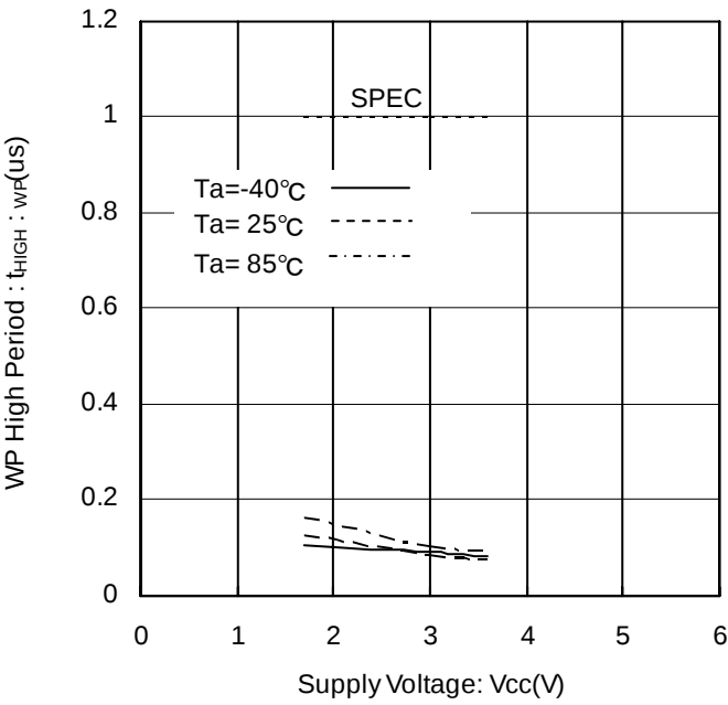
Figure 28. WP High Period vs Supply Voltage
