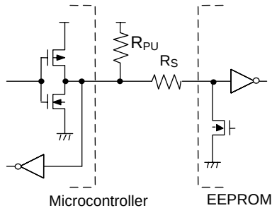
Figure 40. I/O Circuit Diagram
