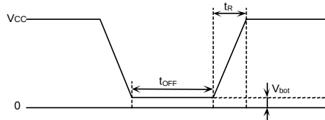
Figure 46. Rise Waveform Diagram
