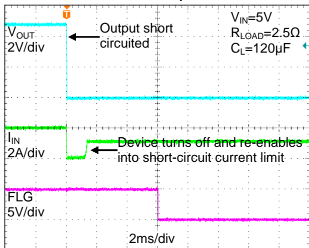
Full-Load to Short-Circuit Transient Response
