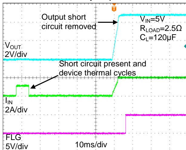
Short-Circuit to Full-Load Recovery Response
