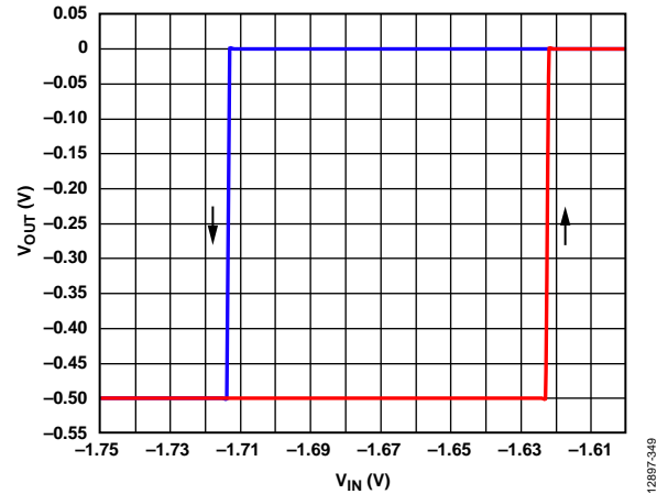
Figure 49. Typical UVLO Behavior, V_{OUT} = -0.5 V
