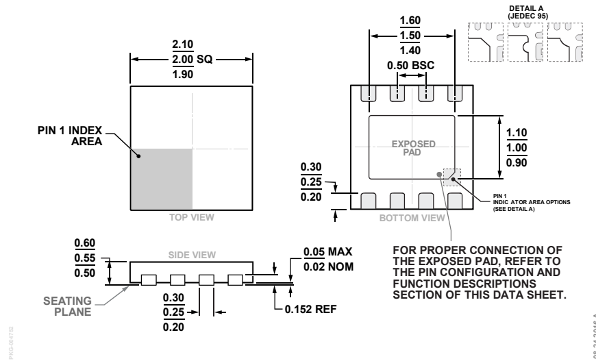
Figure 56. 8-Lead Lead Frame Chip Scale Package [LFCSP] 2 mm x 2 mm Body and 0.55 mm Package Height (CP-8-27) Dimensions shown in millimeters
