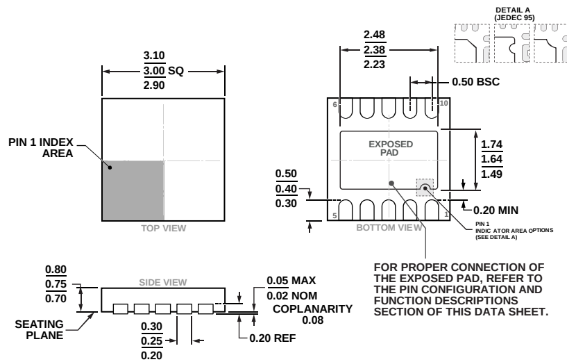
Figure 49. 10-Lead Lead Frame Chip Scale Package [LFCSP]
