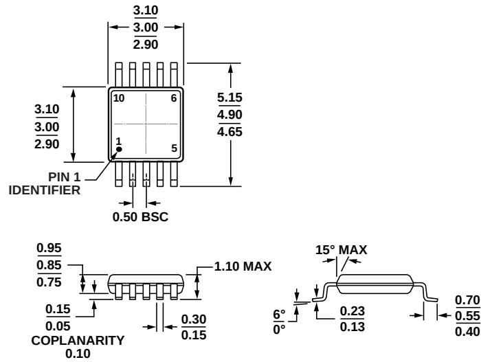
Figure 48. 10-Lead Mini Small Outline Package [MSOP]
