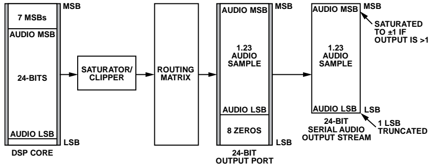
Figure 70. 24-Bit Serial Output Example
