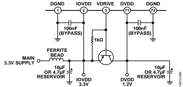
Figure 89. Ferrite Bead Power Supply Isolation Circuit Example
