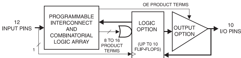
Figure 0-1. Logic Diagram
