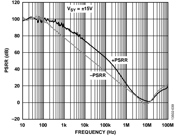
Figure 43. PSRR vs. Frequency, V_{SY} = \pm 15V
