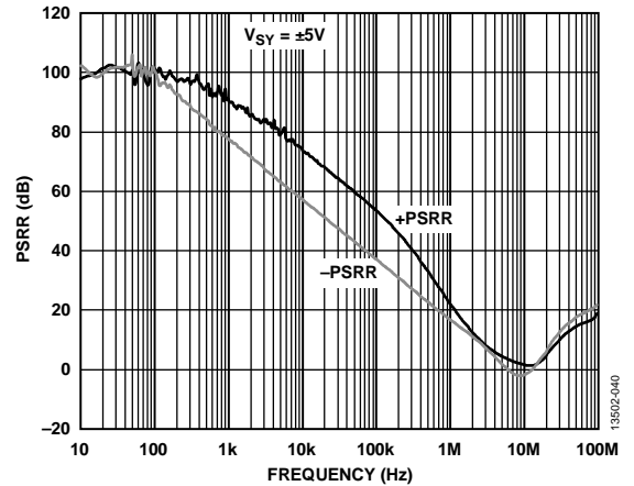
Figure 44. PSRR vs. Frequency, V_{SY} = \pm 5V
