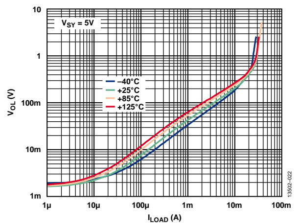
Figure 26. Output Voltage Low ( V_{OL} ) to Supply Rail vs. Load Current ( I_{LOAD} ) over Temperature, V_{SY} = 5 V
