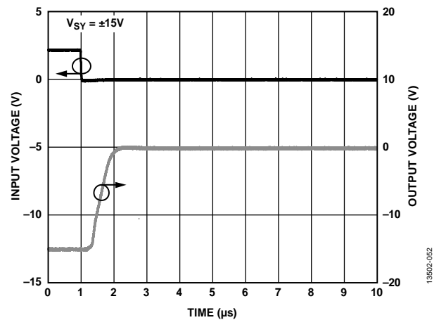
Figure 56. Negative Overload Recovery, A_v = -10 , V_{SY} = \pm 15V
