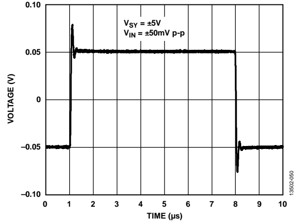
Figure 54. Small Signal Transient Response, V_{SY} = \pm 5V
