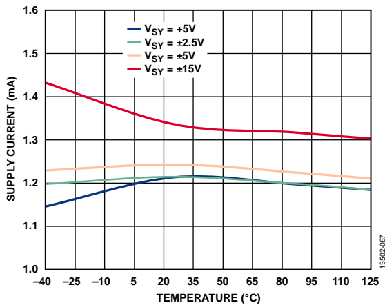
Figure 71. Supply Current ( I_{SY} ) vs. Temperature for Various Supply Voltages
