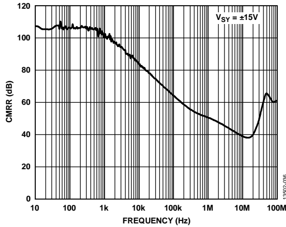
Figure 40. CMRR vs. Frequency, V_{SY} = \pm 15V
