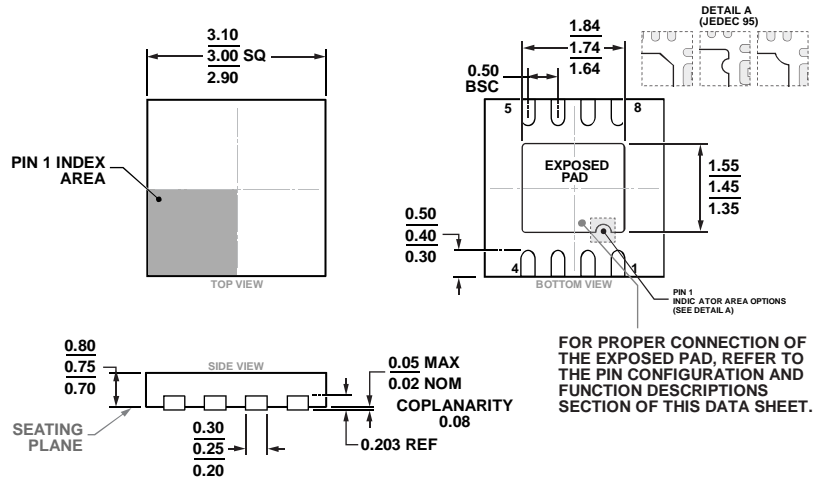
Figure 106. 8-Lead Lead Frame Chip Scale Package [LFCSP] 3 mm x 3 mm Body and 0.75 mm Package Height (CP-8-13)
