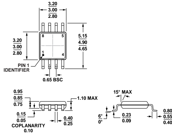
Figure 107. 8-Lead Mini Small Outline Package [MSOP] (RM-8)
