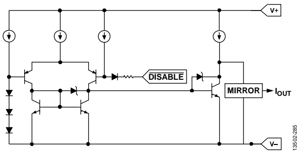
Figure 87. Simplified Circuit for the \overline{\text{DISABLE}} Input
