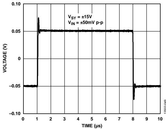
Figure 53. Small Signal Transient Response, V_{SY} = \pm 15V
