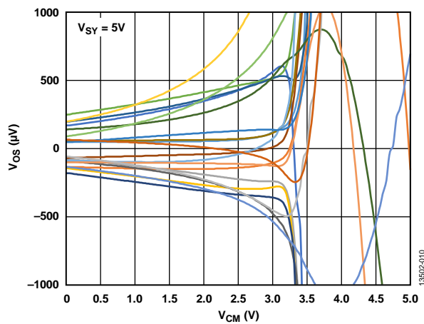
Figure 17. Input Offset Voltage ( V_{OS} ) vs. Common-Mode Voltage ( V_{CM} ), V_{SY} = 5 V
