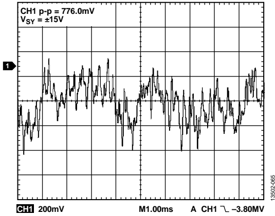
Figure 69. 0.1 Hz to 10 Hz Noise, V_{SY} = \pm 15 V
