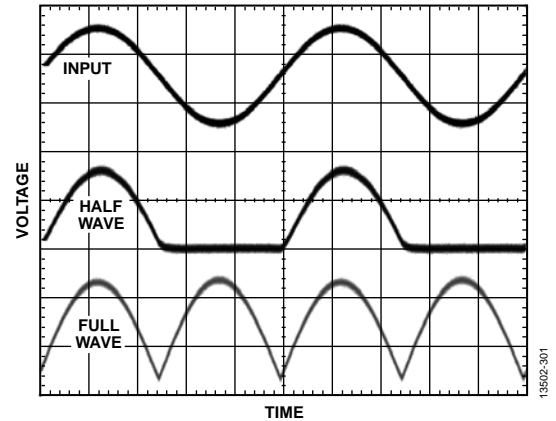
Figure 103. Full Wave and Half Wave Rectifier Input and Output Waveforms
