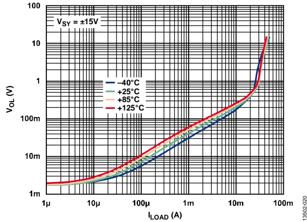
Figure 24. Output Voltage Low ( V_{OL} ) to Supply Rail vs. Load Current ( I_{LOAD} ) over Temperature, V_{SY} = \pm 15 V
