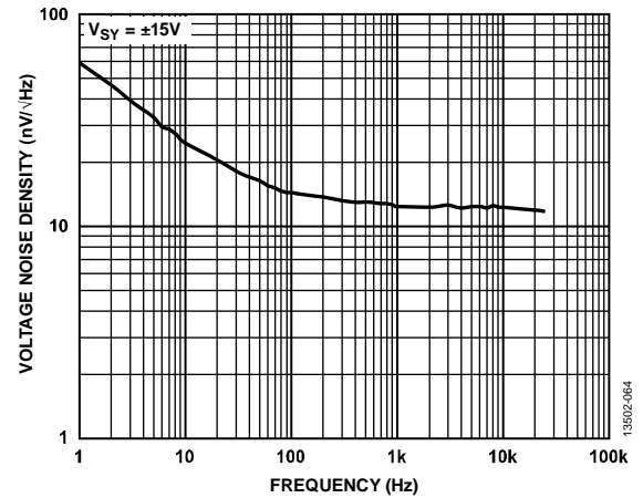
Figure 68. Voltage Noise Density, V_{SY} = \pm 15V
