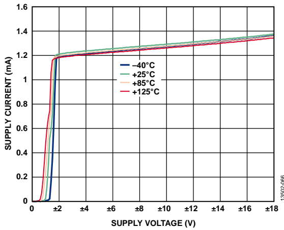
Figure 70. Supply Current ( I_{SY} ) vs. Supply Voltage ( V_{SY} ) for Various Temperatures
