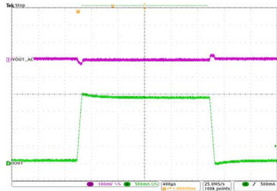
Figure 29. Load Transition (V_{IN}=5.0V, V_{OUT}=1.0V, I_{OUT}=0.1 \text{ to } 2A)
