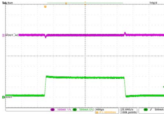
Figure 28. Load Transition (V_{IN}=5.0V, V_{OUT}=1.0V, I_{OUT}=0.1 \text{ to } 1A)
