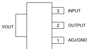
(SOT-223/ H Package)
