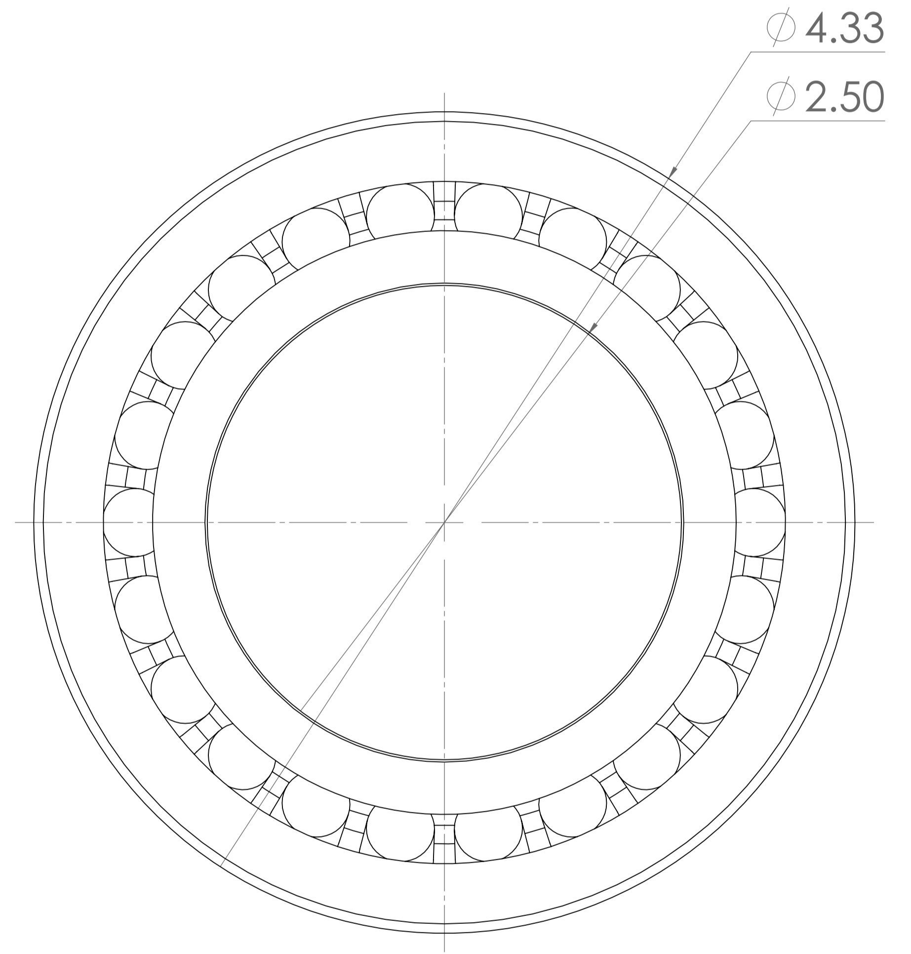
FRONT
