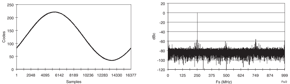
Figure 9-21. F_s = 1 Gps and F_{in} = 250 MHz (Interleaving Mode F_{int} = 2 Gps, F_s/4 DR Type, F_iSDA = -15 ps, ISA = -50 ps)
