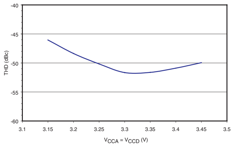
Figure 9-24. THD Versus V_{CCA} = V_{CCD} ( F_s = 1 Gsps, F_{in} = 500 MHz, 1:2 DMUX, F_s/4 DR Type, ISA = -50 ps)
