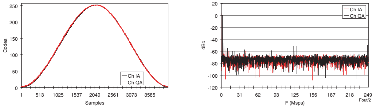
Figure 9-19. F_s = 1 Gps and F_{in} = 1 GHz (1:2 DMUX, F_s/2 DR Type, F_iSDA = -15 ps, ISA = -50 ps)
