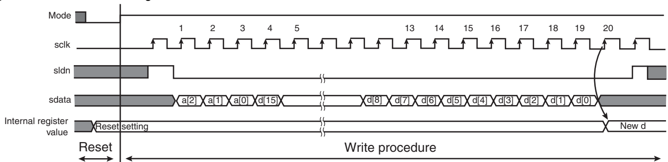
Figure 10-1. Write Chronogram
