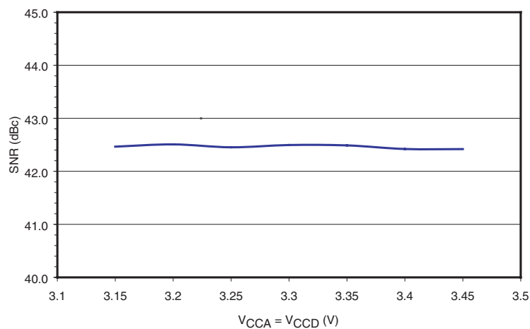
Figure 9-25. SNR Versus V_{CCA} = V_{CCD} ( F_s = 1 Gsps, F_{in} = 500 MHz, 1:2 DMUX, F_s/4 DR Type, ISA = -50 ps)
