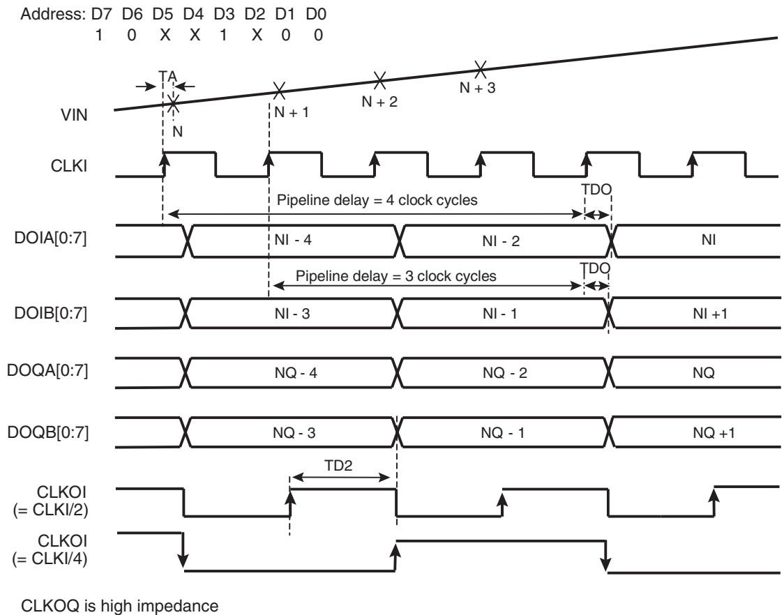
Figure 7-4. 1:2 DMUX Mode, Clock I = ADC I, Clock I = ADC Q
