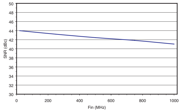
Figure 9-16. SNR Versus Input Frequency ( F_s = 1 Gsps)
