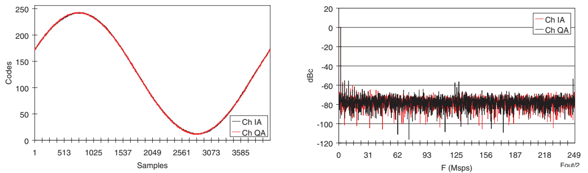
Figure 9-18. F_s = 1 Gsps and F_{in} = 500 MHz (1:2 DMUX, F_s/2 DR Type, F_iSDA = -15 ps, ISA = -50 ps)
