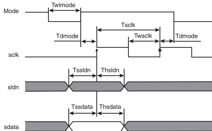
Figure 10-2. Timing Definition
