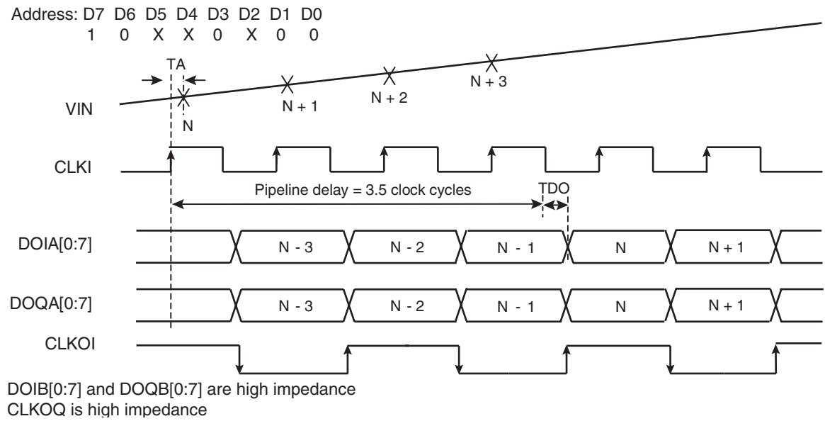
Figure 7-5. 1:1 DMUX Mode, Clock I = ADC I, Clock I = ADC Q
