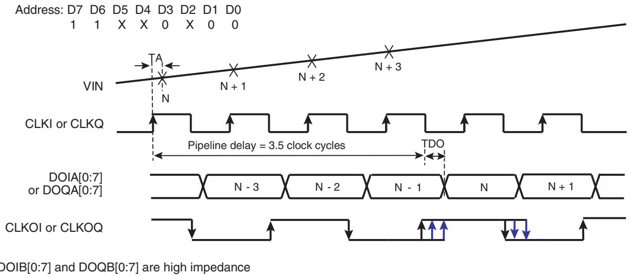
Figure 7-3. 1:1 DMUX Mode, Clock I = ADC I, Clock Q = ADC Q
