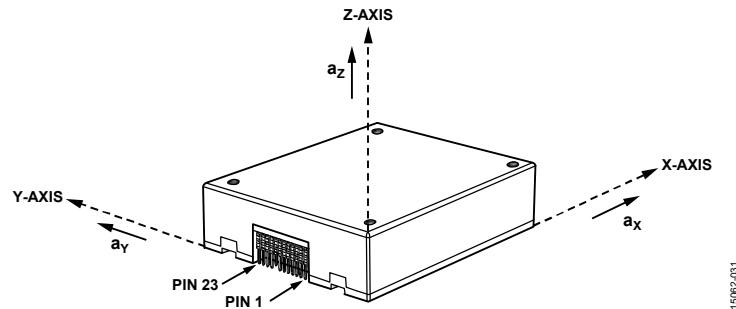
Figure 31. Accelerometer Axis and Polarity Assignments
