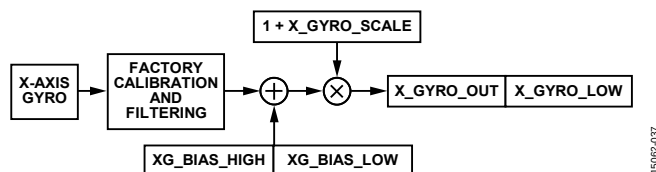
Figure 37. User Bias/Scale Adjustment Registers in Gyroscopic Signal Path
