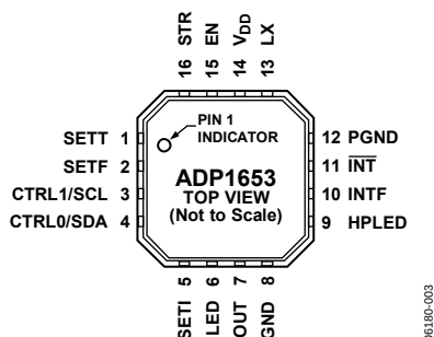
Figure 4. Pin Configuration
