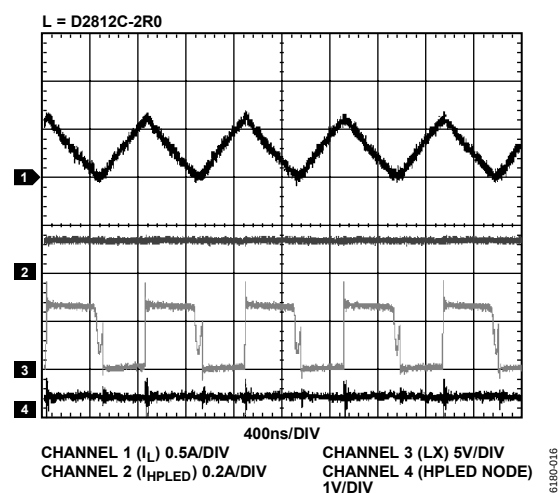
Figure 10. Inductor Current, Two LEDs Torch Mode, LED Current = 130 mA, V_{DD} = 3.6\text{ V}
