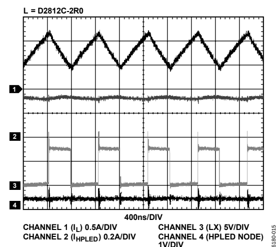
Figure 9. Inductor Current, Two LEDs Flash Mode, LED Current = 335 mA, V_{DD} = 3.6\text{ V}
