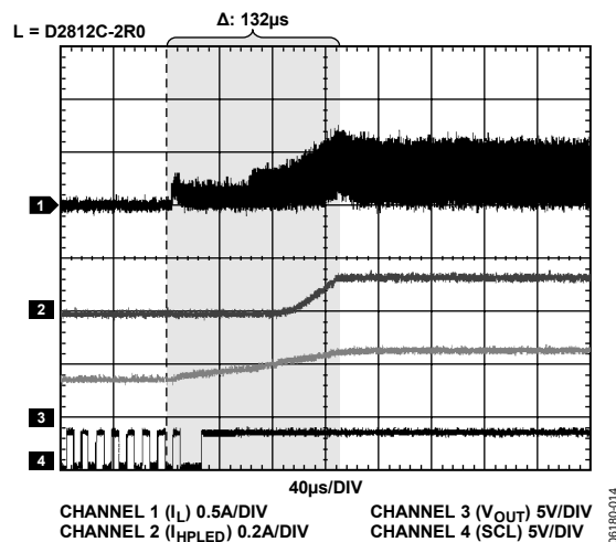
Figure 8. Startup, Two LEDs Torch Mode, LED Current = 130 mA, V_{DD} = 3.6\text{ V}
