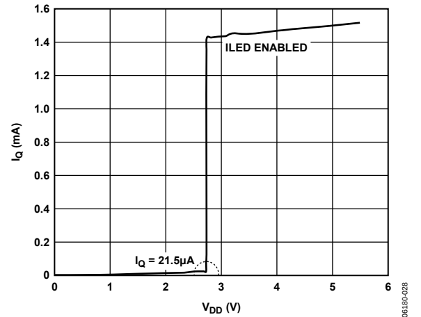
Figure 21. Quiescent Current vs. V_{DD} , V_{DD} Swept from 5.5 V to 0 V, ILED Active at 2.5 mA Until UVLO Threshold
