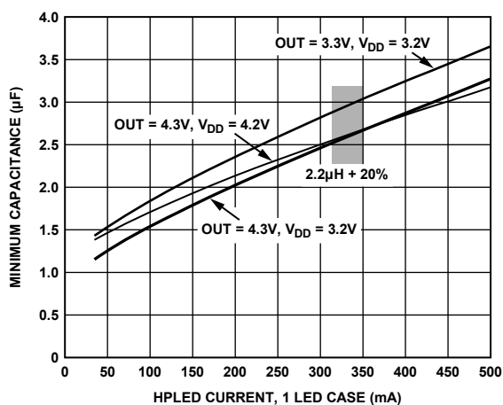
Figure 32. Minimum Output Capacitance for L = 2.2 \mu\text{H} + 20\% for One-LED Design
