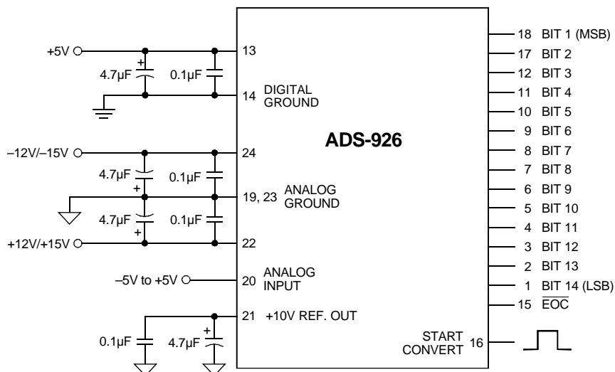
Figure 3. Typical ADS-926 Connection Diagram
