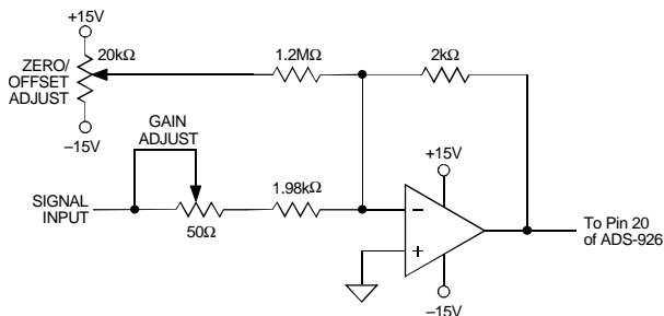
Figure 2. ADS-926 Calibration Circuit
