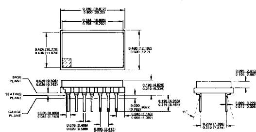
14-Pin Dual-In-Line Ceramic Package
