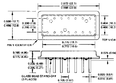
14-Pin Dual-In-Line Metal Package
