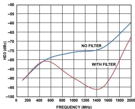
Figure 48. HD3 vs. Frequency, With and Without LC Filter
