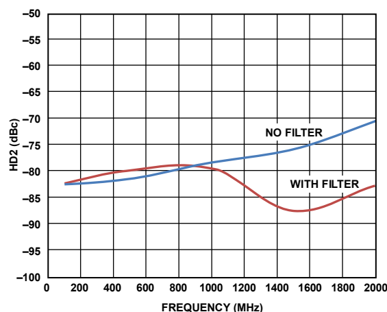
Figure 47. HD2 vs. Frequency, With and Without LC Filter
