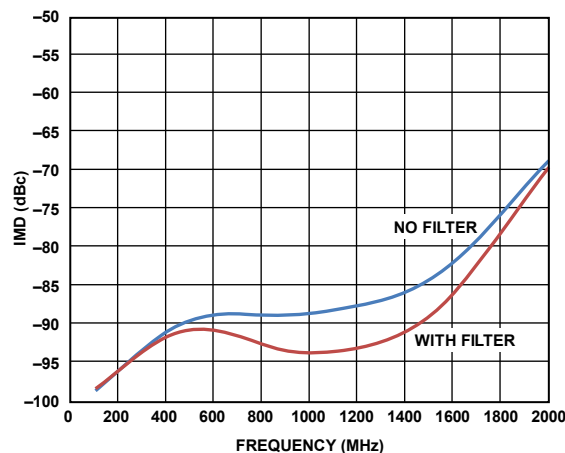
Figure 46. IMD vs. Frequency, With and Without LC Filter
