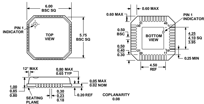
Figure 81. 40-Lead Lead Frame Chip Scale Package [LFCSP_VQ]
