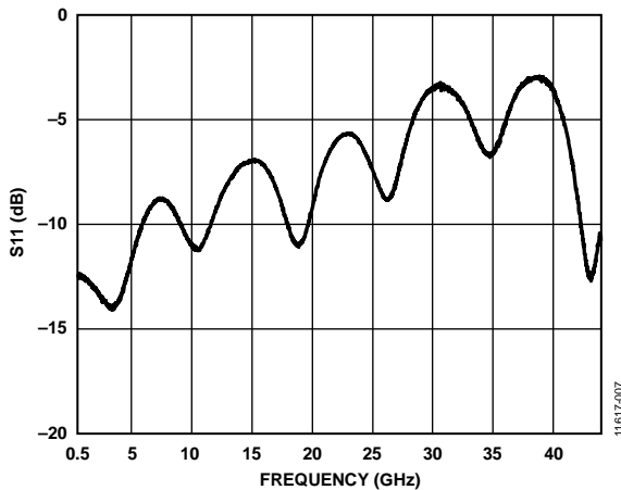
Figure 5. Input Return Loss (S 11 ) vs. Input Frequency with Input Connector and PCB Trace Embedded
