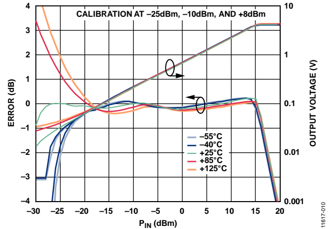
Figure 8. Conformance Error and Output Voltage (V OUT ) vs. RF Input Power (P IN ) for Various Temperatures at 1 GHz
