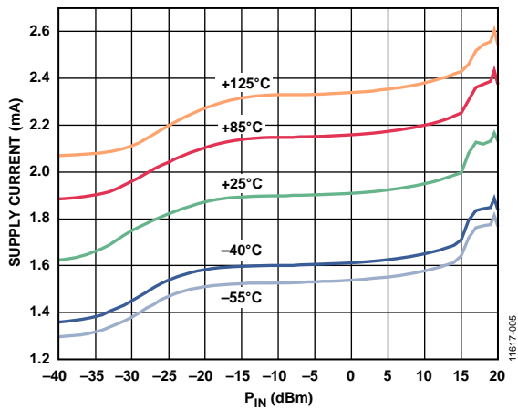
Figure 4. Supply Current vs. RF Input Power (P IN ) for Various Temperatures
