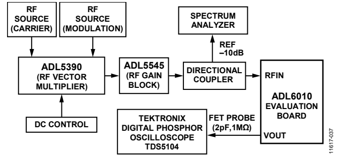
Figure 36. Hardware Configuration for Envelope Output Response Measurement
