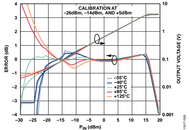
Figure 7. Conformance Error and Output Voltage (V OUT ) vs. RF Input Power (P IN ) for Various Temperatures at 0.5 GHz
