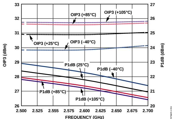
Figure 26. OIP3 and P1dB vs. Frequency and Temperature, 3.3 V Supply, 2.5 GHz to 2.7 GHz
