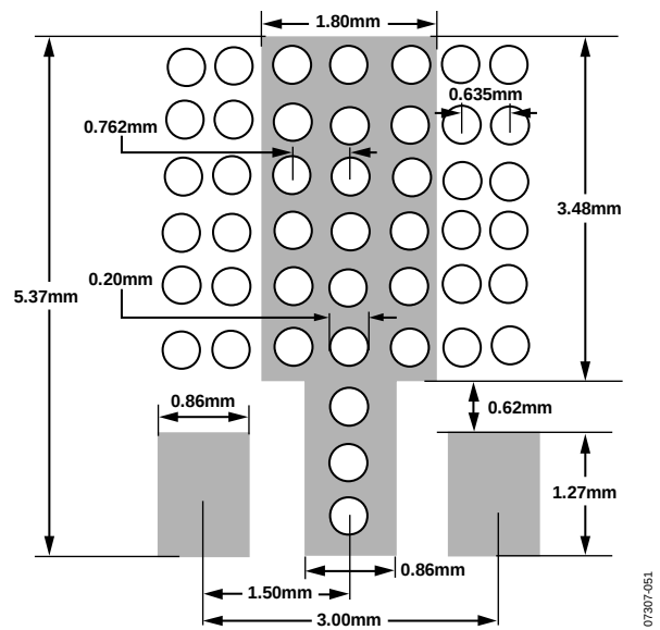
Figure 29. Recommended Land Pattern
