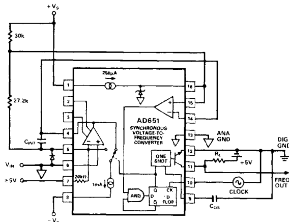
Figure 8. Bipolar Offset
