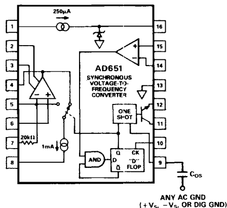
Figure 12. One Shot Enabled
