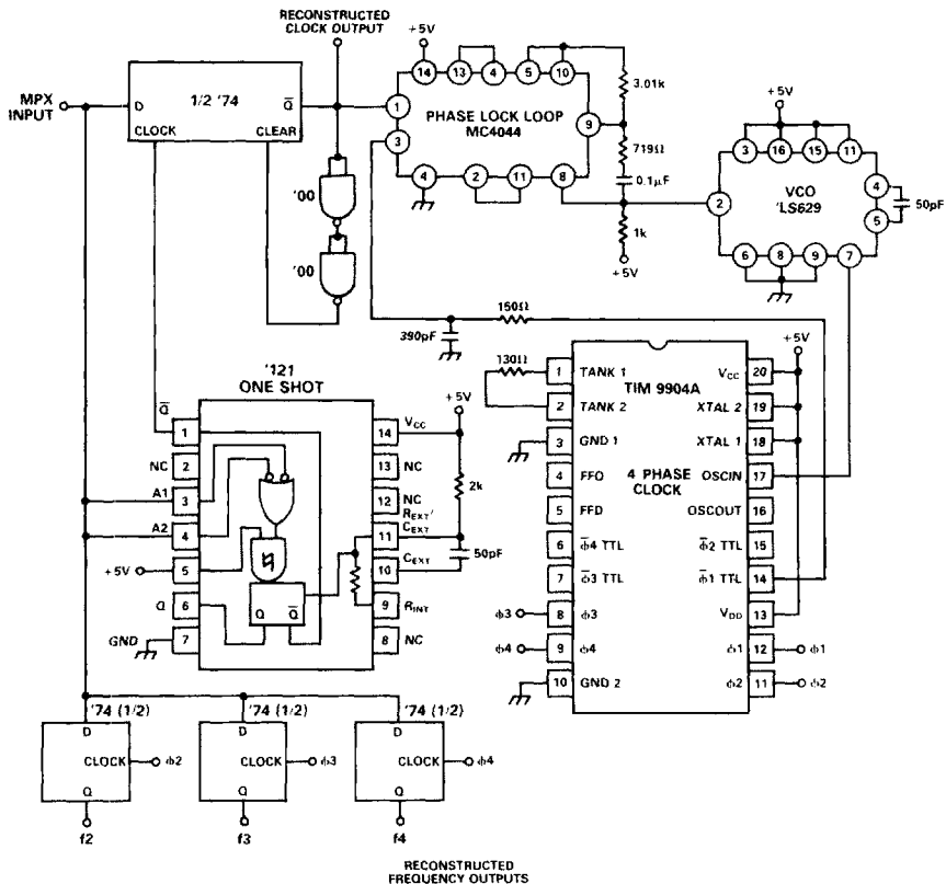
Figure 22. SVFC Demultiplexers
