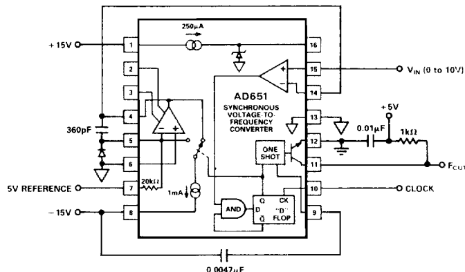
Figure 28. Delta Modulator
