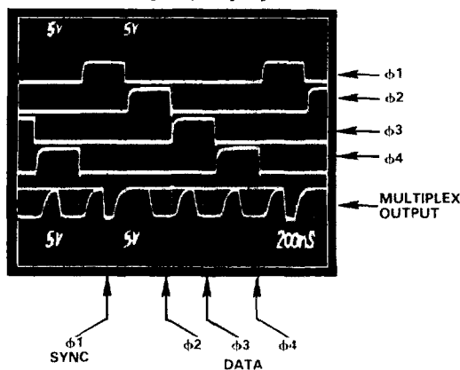
Figure 23. Multiplexer Waveforms
