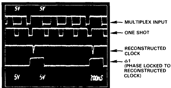
Figure 24. Demultiplexer Waveforms
