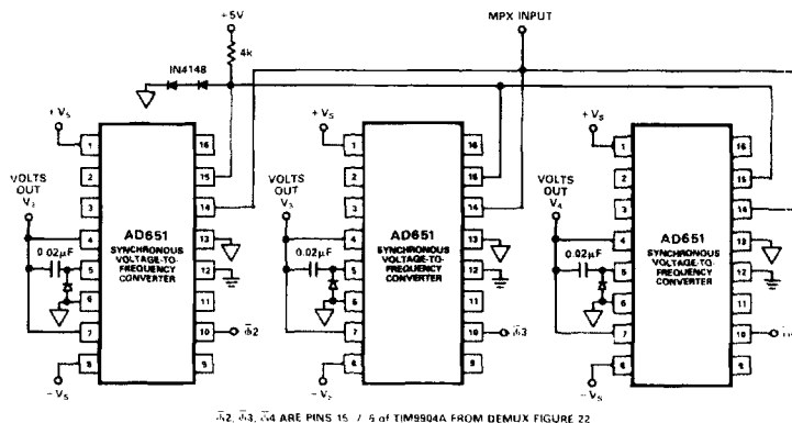
Figure 25. Demultiplexer Frequency-to-Voltage Conversion
