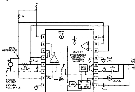
Figure 15. Single Supply Negative Voltage Input
