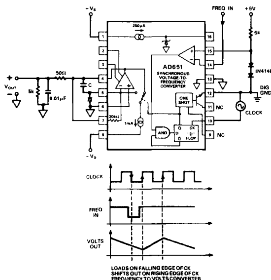
Figure 16. Frequency-to-Voltage Converter
