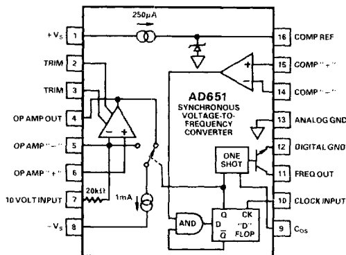
Figure 1. AD651 Pin Configuration
