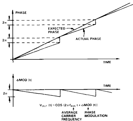
Figure 5. Phase Modulation
