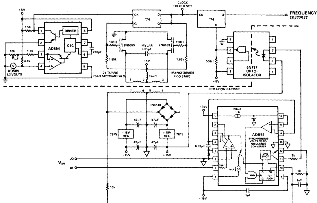
Figure 26. Isolated Synchronous VFC
