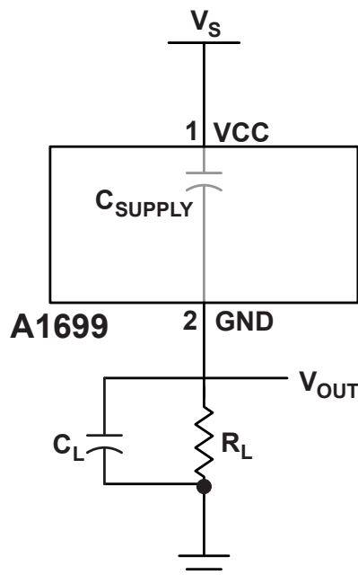
Figure 1: Typical Application Circuit
