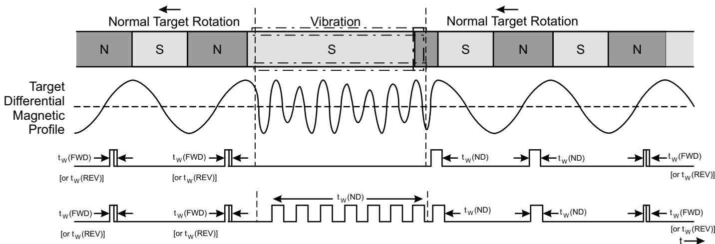
Figure 13: Output Functionality in the Presence of Running Mode Target Vibration (-xxxxH variant)
