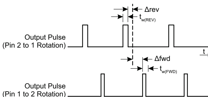
Figure 7: Output Protocol (-FDxxxx variant)
