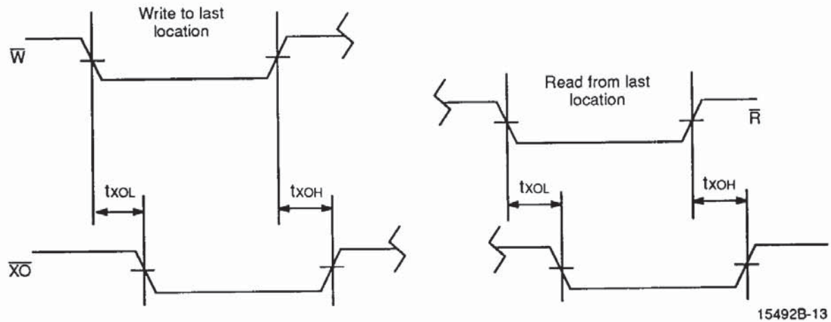
Figure 10. \overline{X0} Delay from Clock
