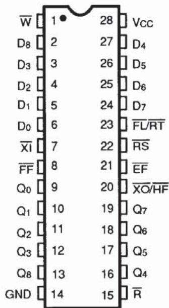
DIPs*
