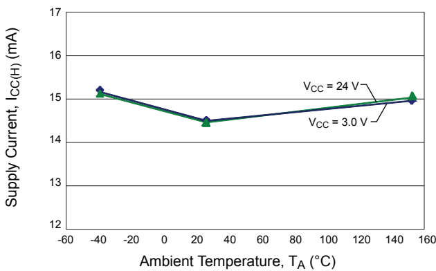
A1190, A1192, A1193 Average Supply Current (High) versus Temperature
