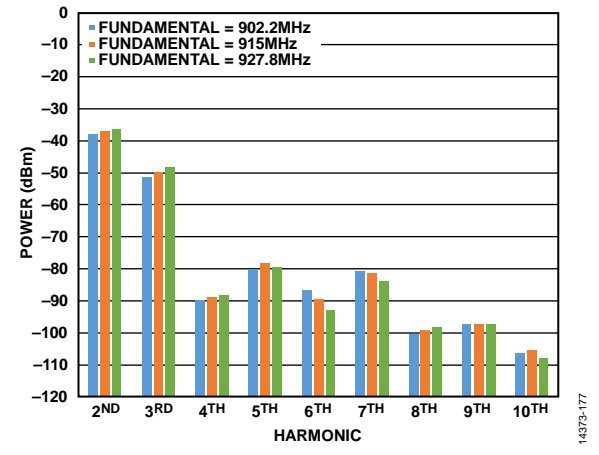
Figure 78. Conductive Harmonic Emission Level, PA2 Output Power = 17 dBm, RF Frequency = 915 MHz, V_{DD} = 3.0\text{ V} , T_A = 25^\circ\text{C}
