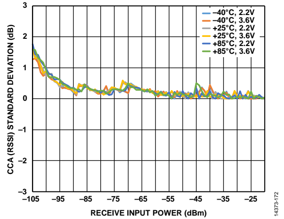
Figure 73. CCA (RSSI) Standard Deviation vs. Rx Input Power, Temperature and V_{DD} , with One-Point Calibration at -70 dBm ( V_{DD} = 2.2 V, T_A = 25^\circ\text{C} ); Unmodulated RF Signal; Configuration 915 MHz/150 kbps (Standard Deviation is Based on 100 CCA Operations)
