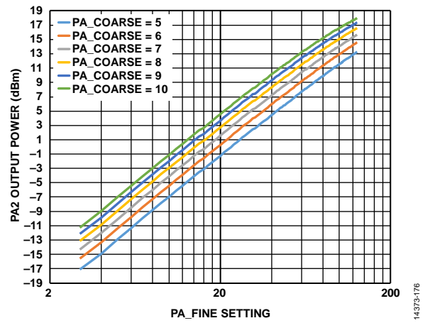
Figure 77. PA2 Output Power vs. PA_FINE Setting and PA_COARSE Setting with PA_FINE on a Logarithmic Scale, PAOLDO_VOUT_CON = 15, RF Frequency = 915 MHz, V_{DD} = 3.0\text{ V} , T_A = 25^\circ\text{C}
