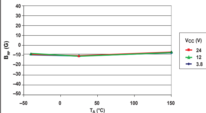
Release Point versus Ambient Temperature
