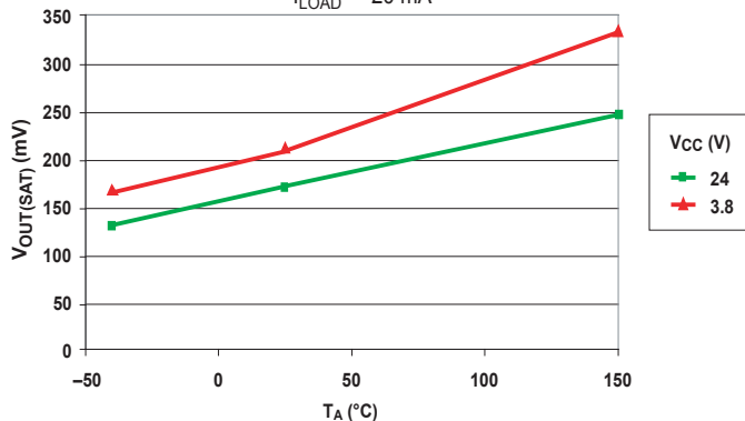
Output Voltage (On) versus Ambient Temperature
