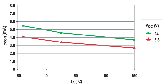
Supply Current (Off) versus Ambient Temperature
