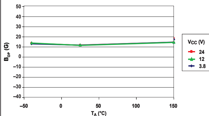
Operate Point versus Ambient Temperature
