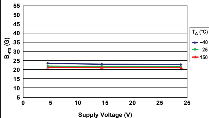
Hysteresis versus Supply Voltage
