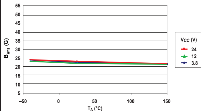
Hysteresis versus Ambient Temperature
