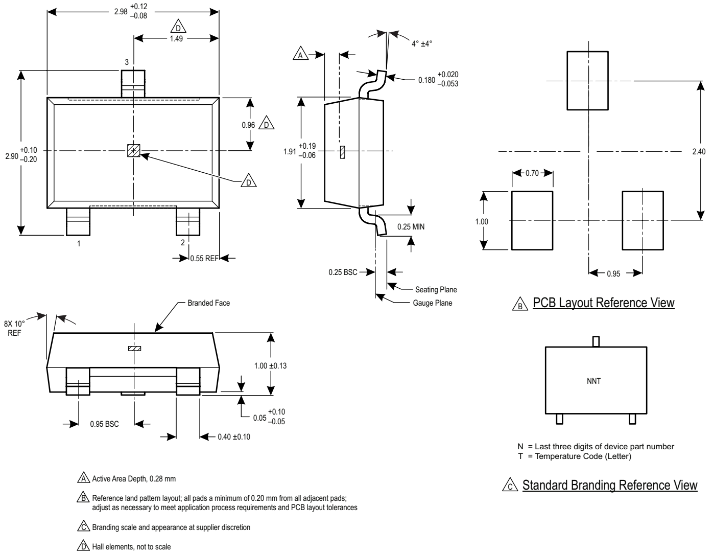
Figure 3: Package LH, 3-Pin (SOT-23W)
